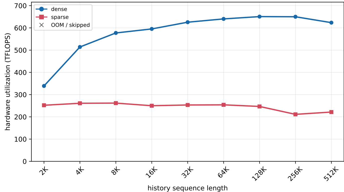
H800 MLA prefill - batch=32, new length=2 (chunked prefill)
