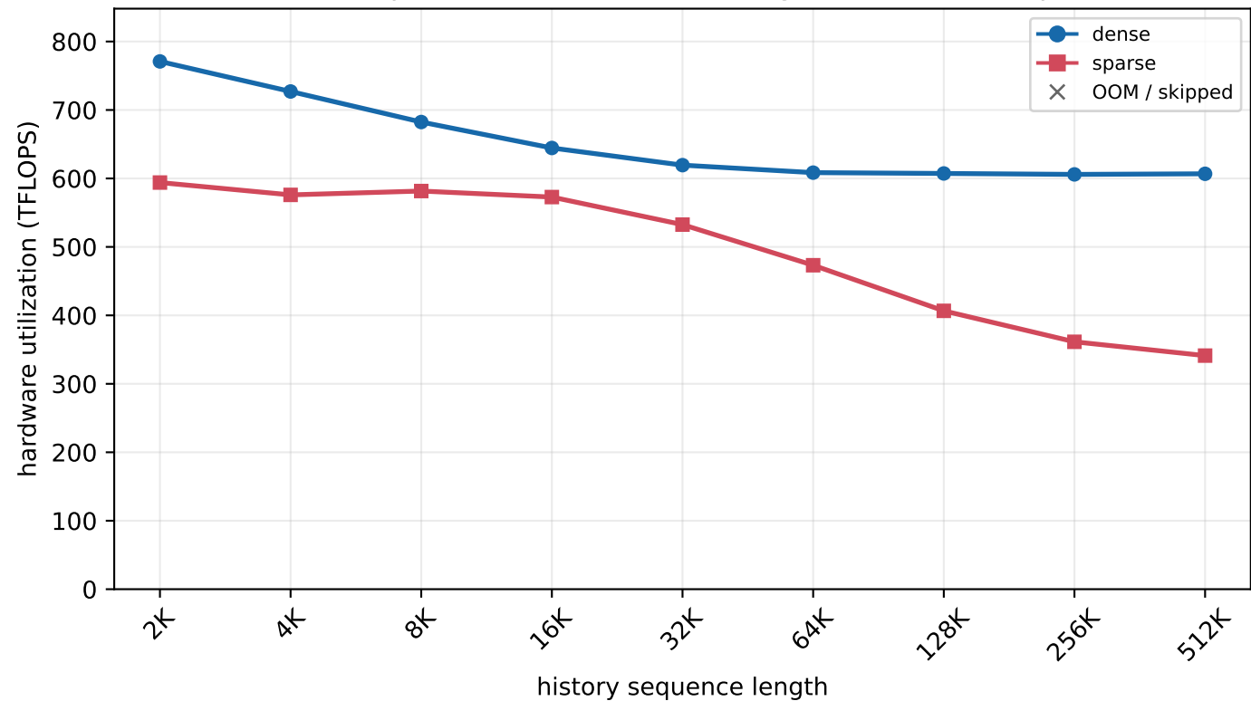
H800 MLA prefill - batch=32, new length=2K (chunked prefill)
