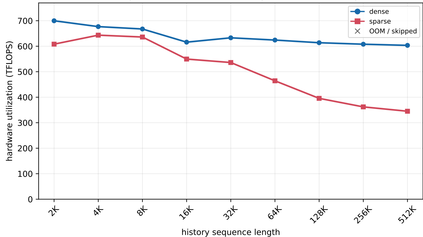
H800 MLA prefill - batch=32, new length=256 (chunked prefill)
