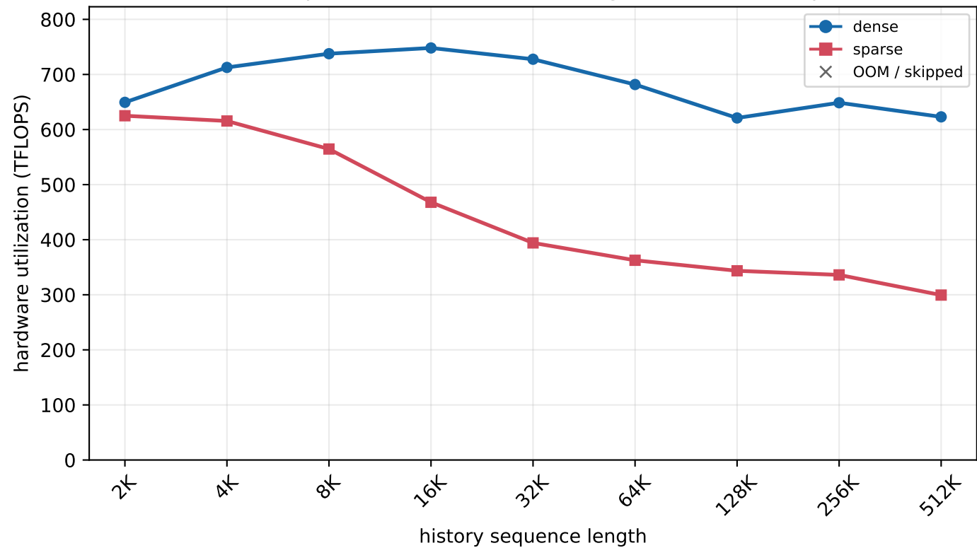
H800 MLA prefill - batch=32, new length=32 (chunked prefill)
