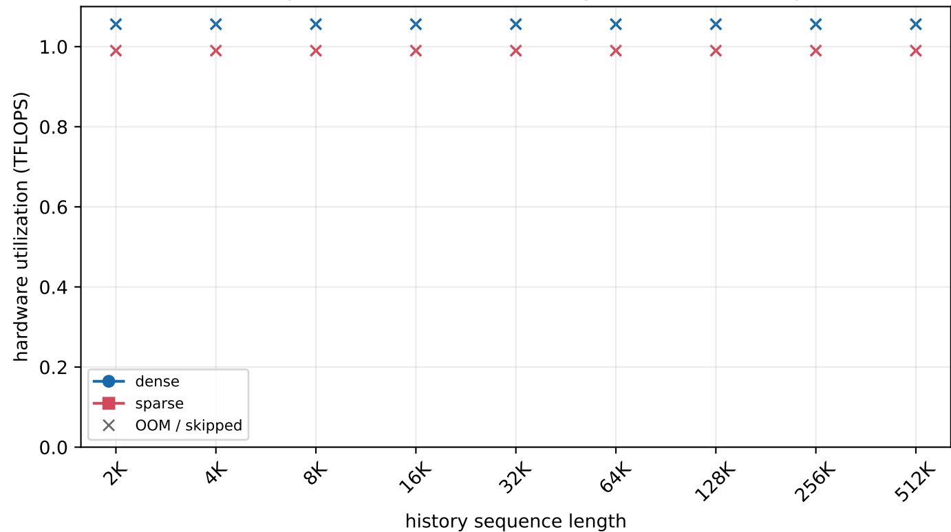
H800 MLA prefill - batch=32, new length=32K (chunked prefill)
