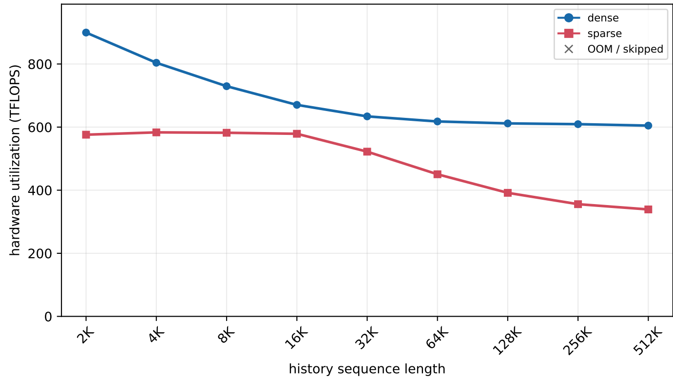
H800 MLA prefill - batch=32, new length=4K (chunked prefill)
