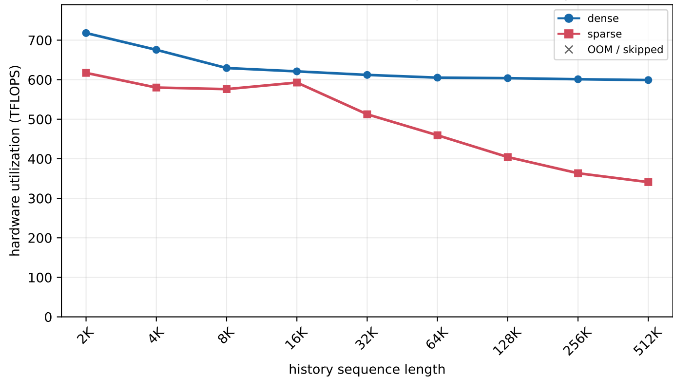
H800 MLA prefill - batch=32, new length=512 (chunked prefill)
