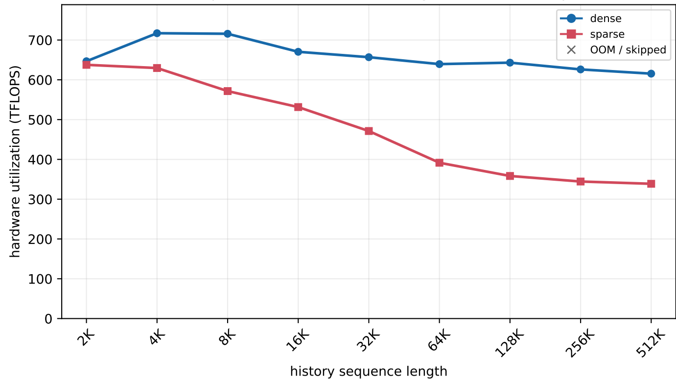
H800 MLA prefill - batch=32, new length=64 (chunked prefill)
