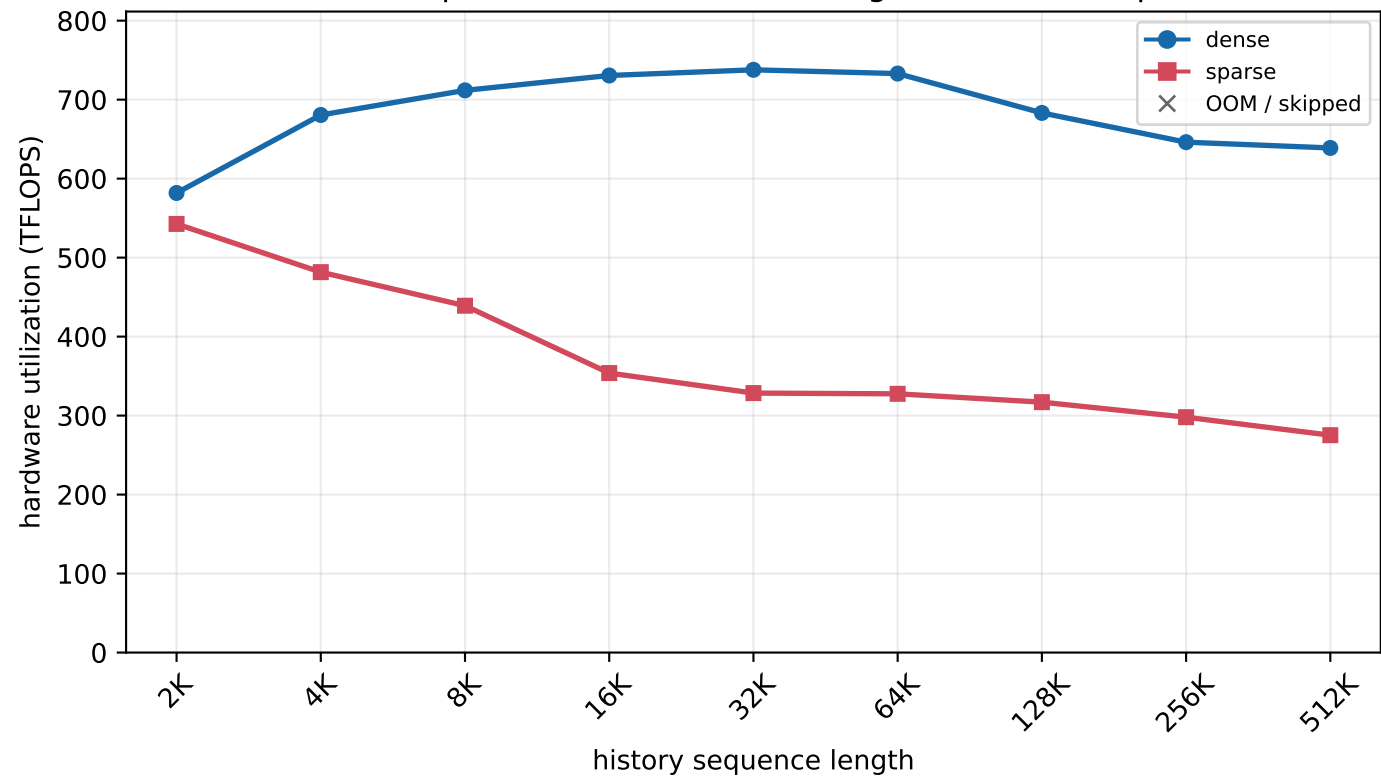
H800 MLA prefill - batch=32, new length=8 (chunked prefill)
