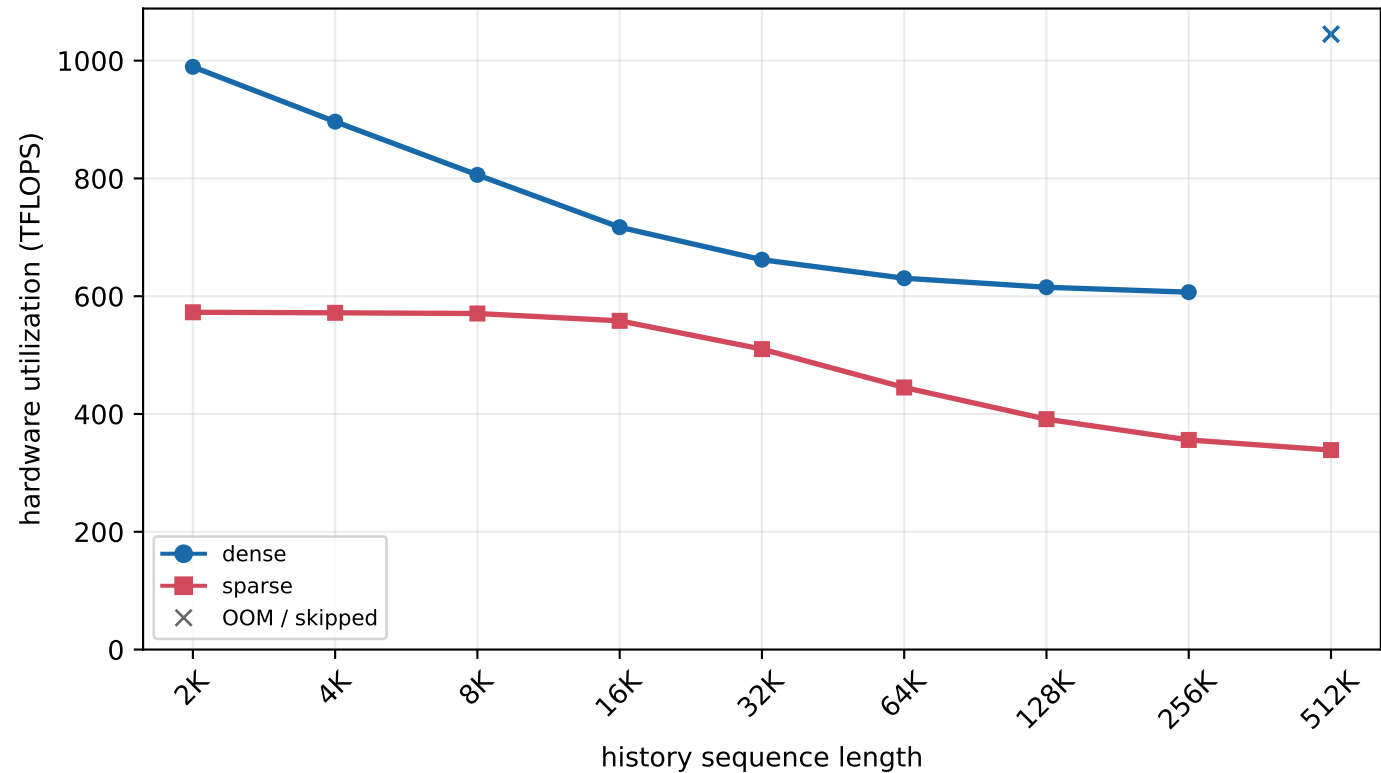
H800 MLA prefill - batch=32, new length=8K (chunked prefill)
