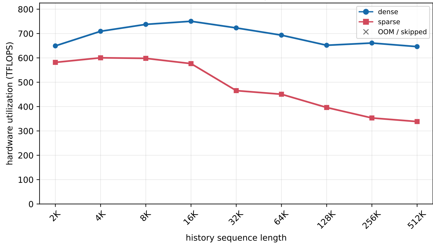
H800 MLA prefill - batch=4, new length=128 (chunked prefill)
