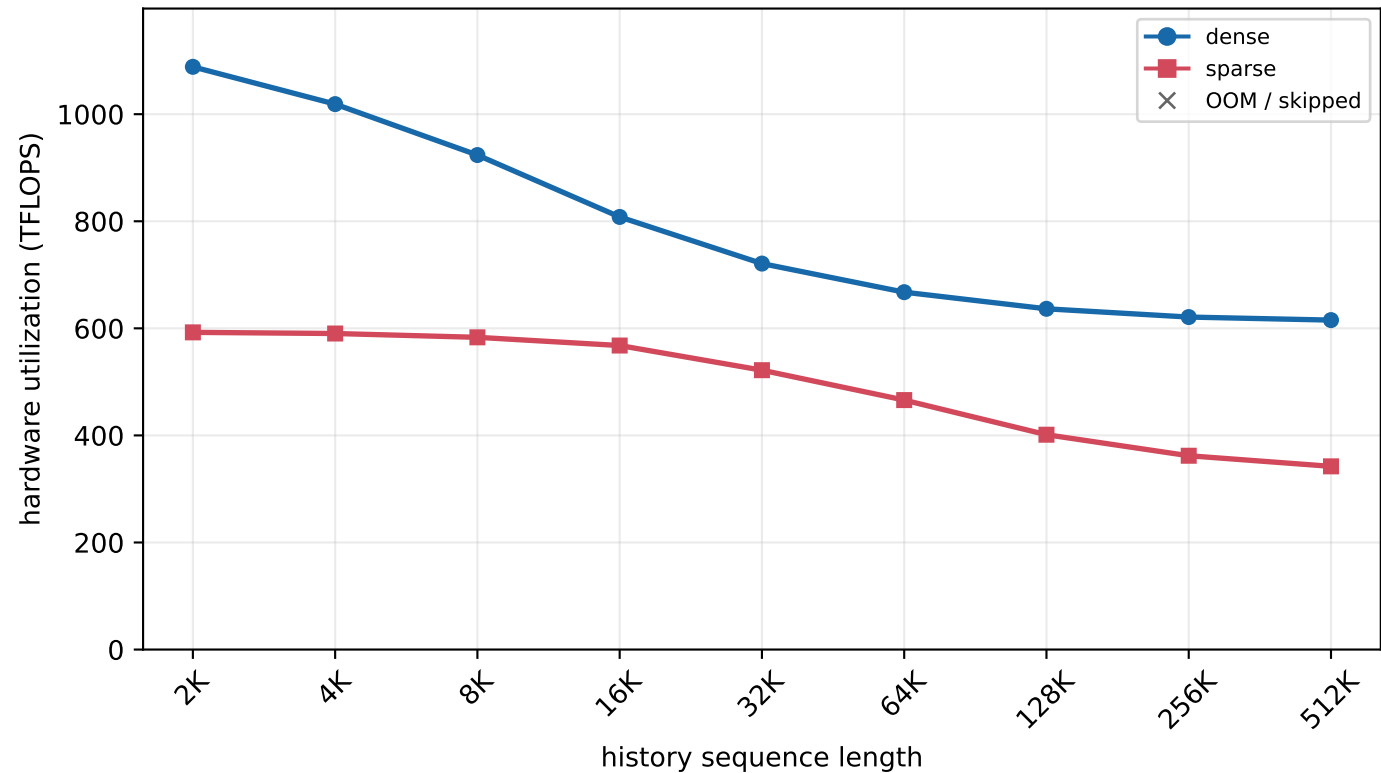
H800 MLA prefill - batch=4, new length=16K (chunked prefill)
