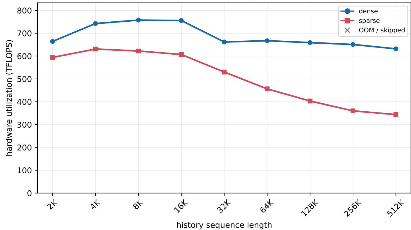
H800 MLA prefill - batch=4, new length=256 (chunked prefill)
