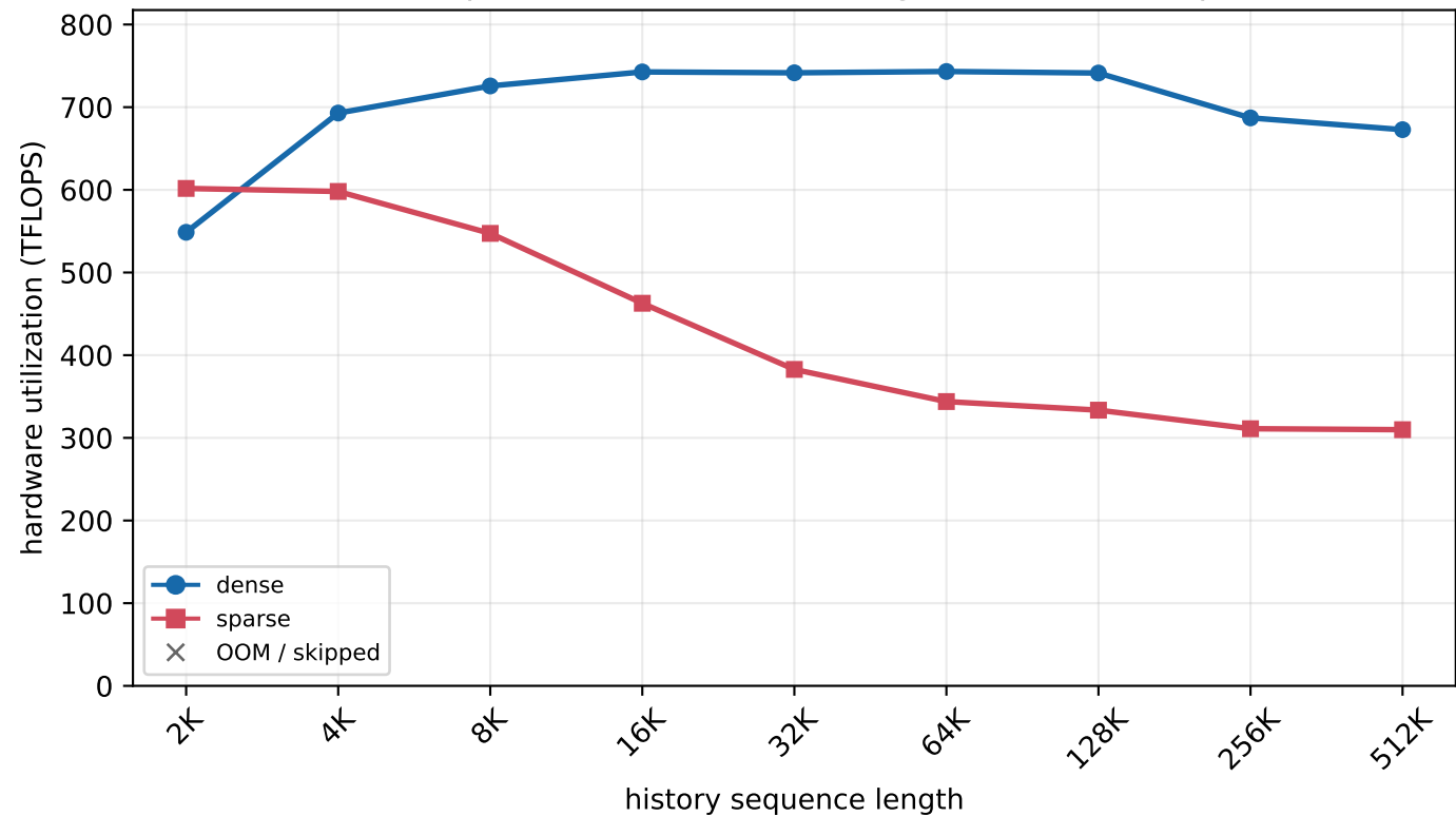
H800 MLA prefill - batch=4, new length=32 (chunked prefill)
