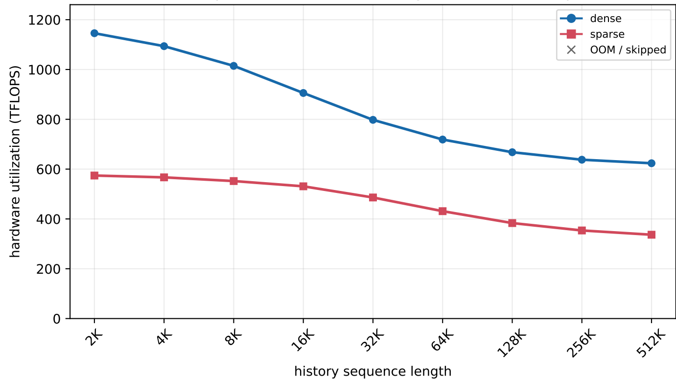
H800 MLA prefill - batch=4, new length=32K (chunked prefill)
