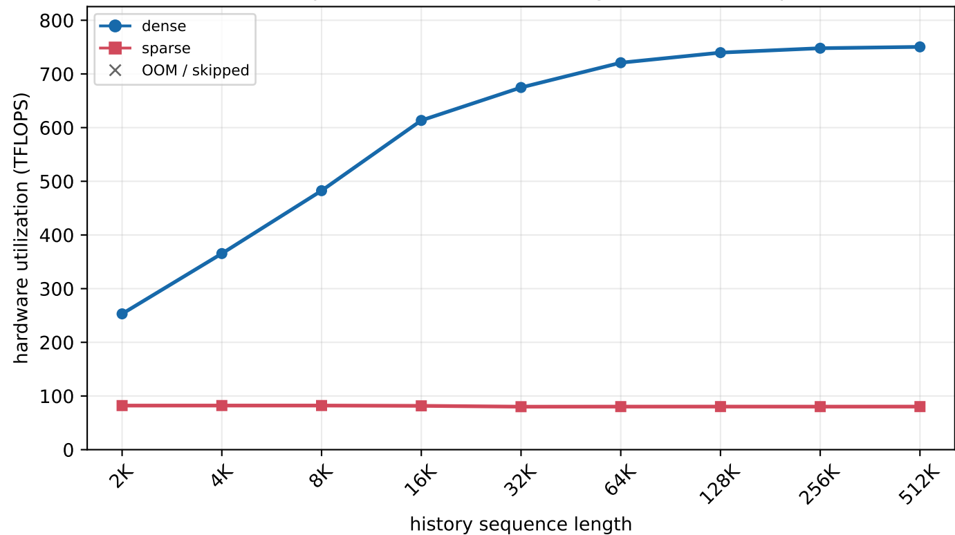
H800 MLA prefill - batch=4, new length=4 (chunked prefill)
