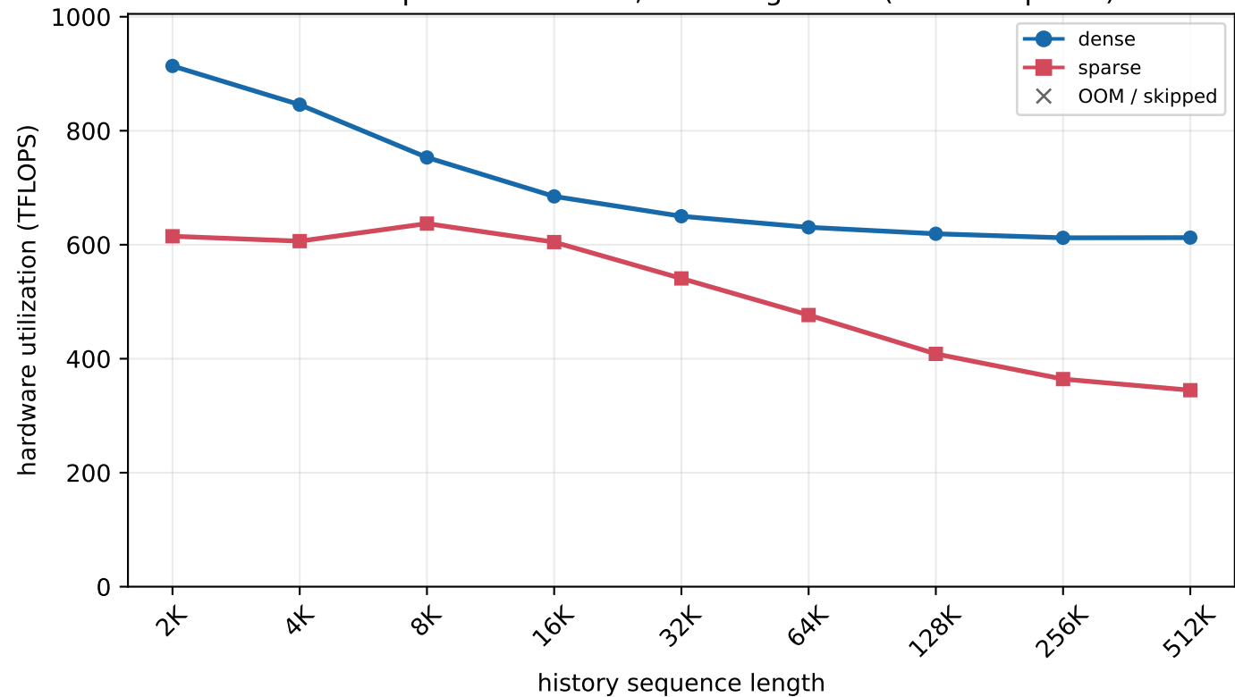
H800 MLA prefill - batch=4, new length=4K (chunked prefill)
