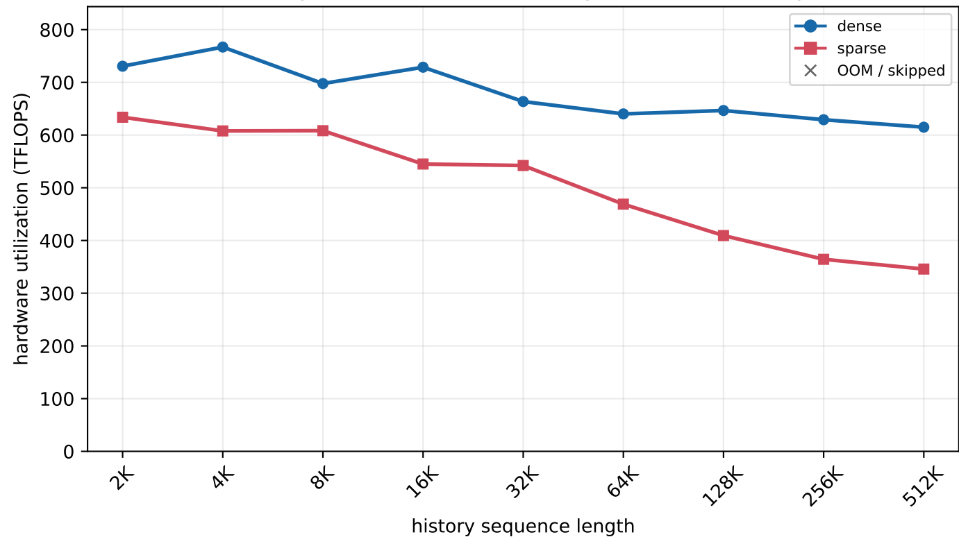
H800 MLA prefill - batch=4, new length=512 (chunked prefill)
