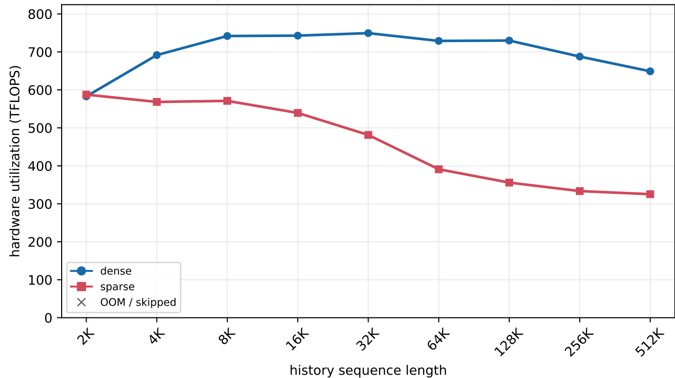
H800 MLA prefill - batch=4, new length=64 (chunked prefill)
