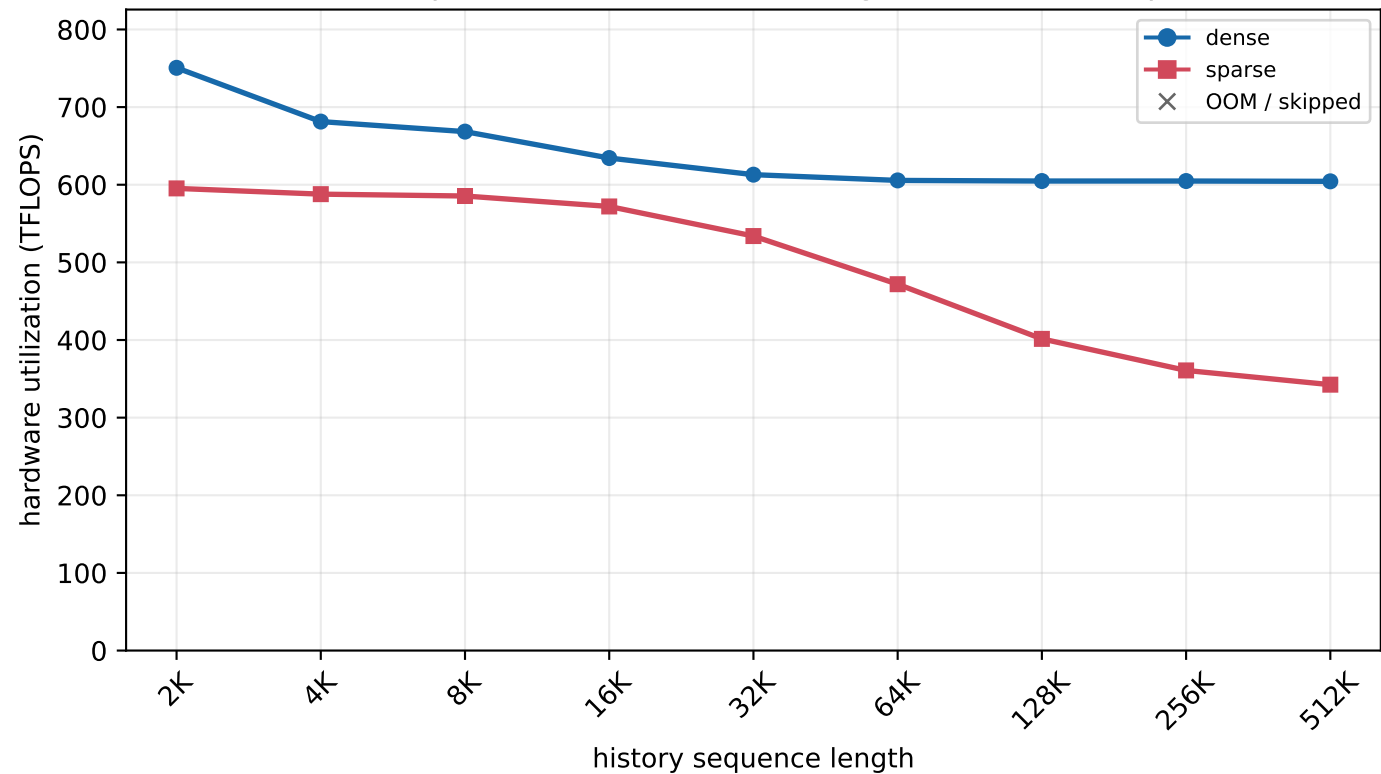
H800 MLA prefill - batch=64, new length=1K (chunked prefill)
