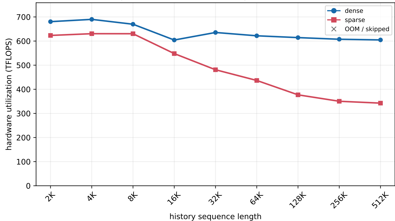
H800 MLA prefill - batch=64, new length=128 (chunked prefill)
