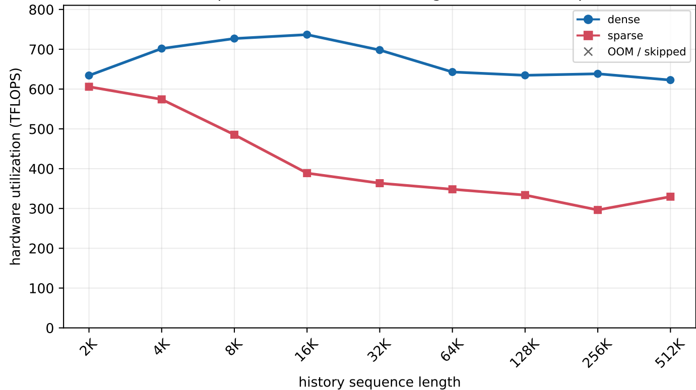
H800 MLA prefill - batch=64, new length=16 (chunked prefill)
