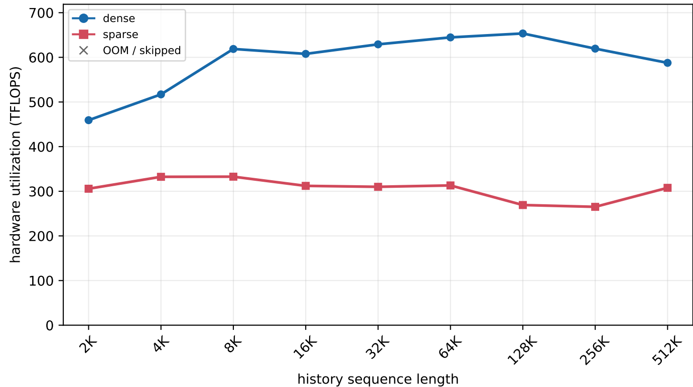
H800 MLA prefill - batch=64, new length=2 (chunked prefill)
