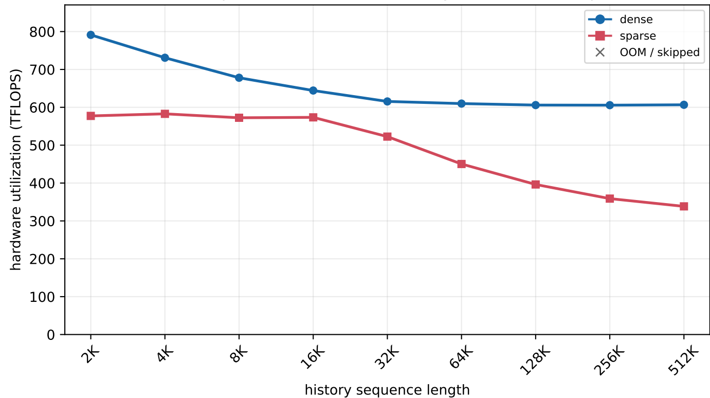
H800 MLA prefill - batch=64, new length=2K (chunked prefill)
