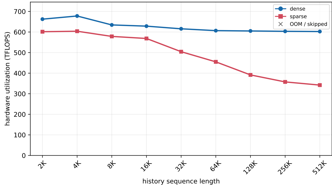
H800 MLA prefill - batch=64, new length=256 (chunked prefill)
