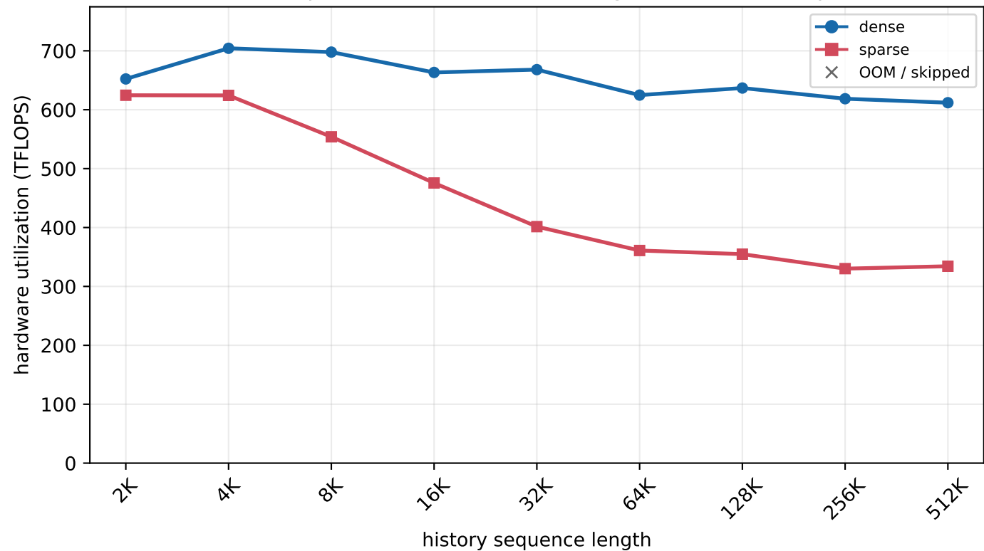
H800 MLA prefill - batch=64, new length=32 (chunked prefill)
