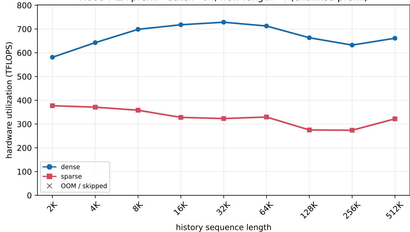
H800 MLA prefill - batch=64, new length=4 (chunked prefill)
