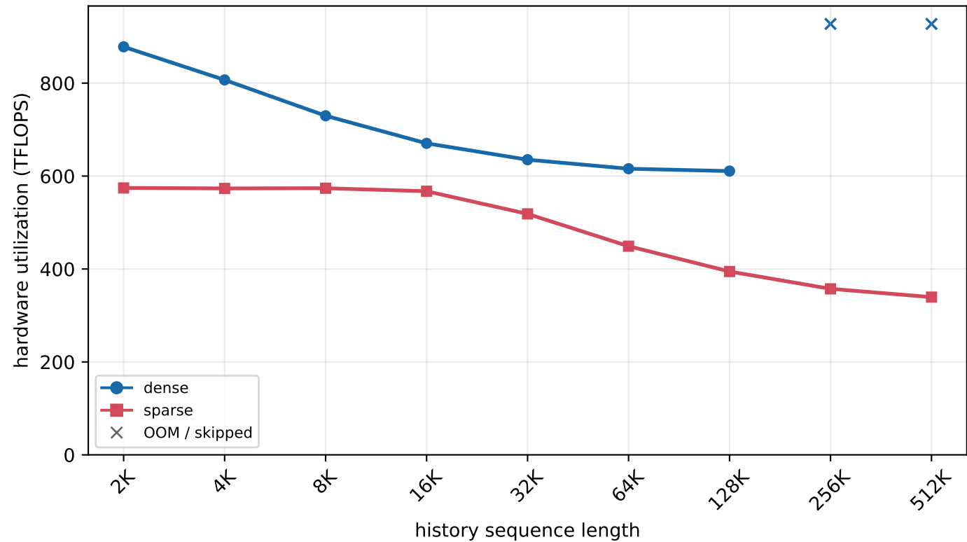
H800 MLA prefill - batch=64, new length=4K (chunked prefill)
