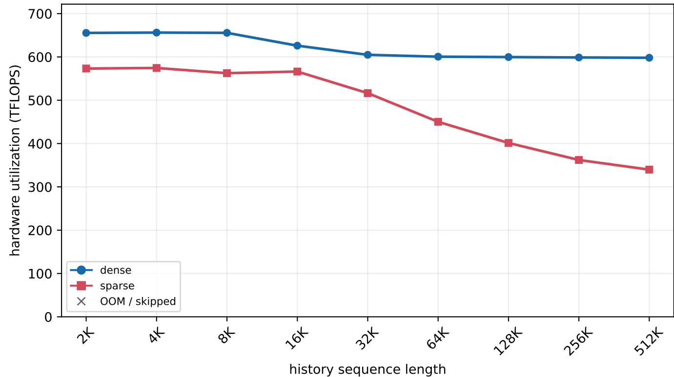
H800 MLA prefill - batch=64, new length=512 (chunked prefill)
