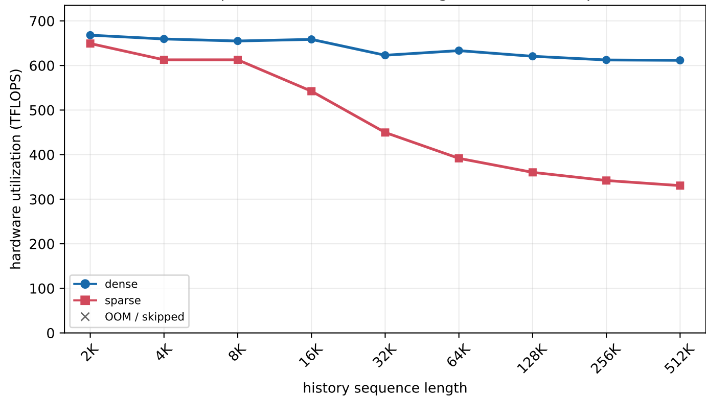
H800 MLA prefill - batch=64, new length=64 (chunked prefill)
