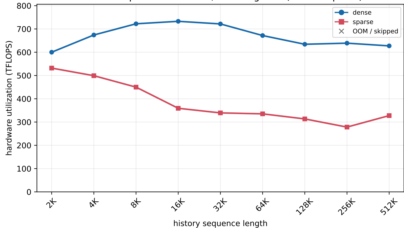
H800 MLA prefill - batch=64, new length=8 (chunked prefill)
