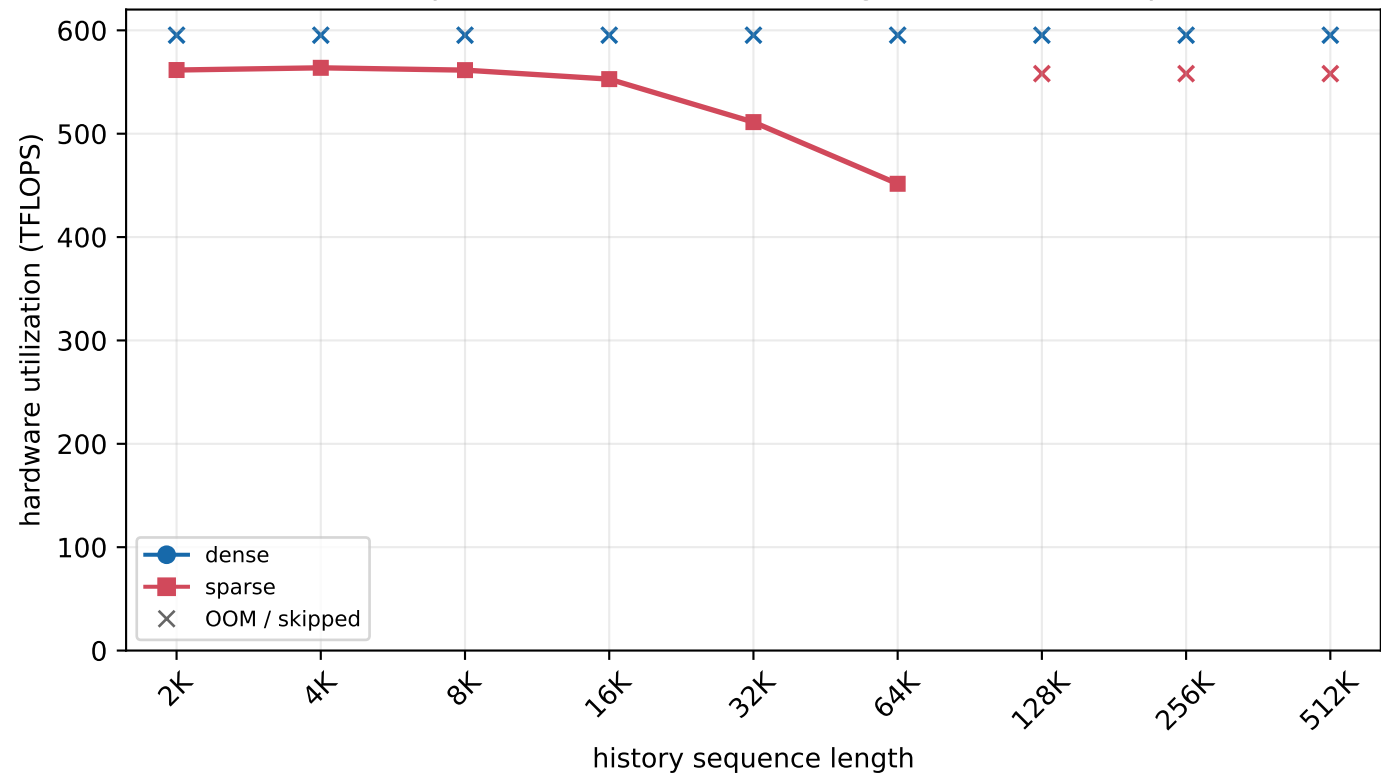
H800 MLA prefill - batch=64, new length=8K (chunked prefill)
