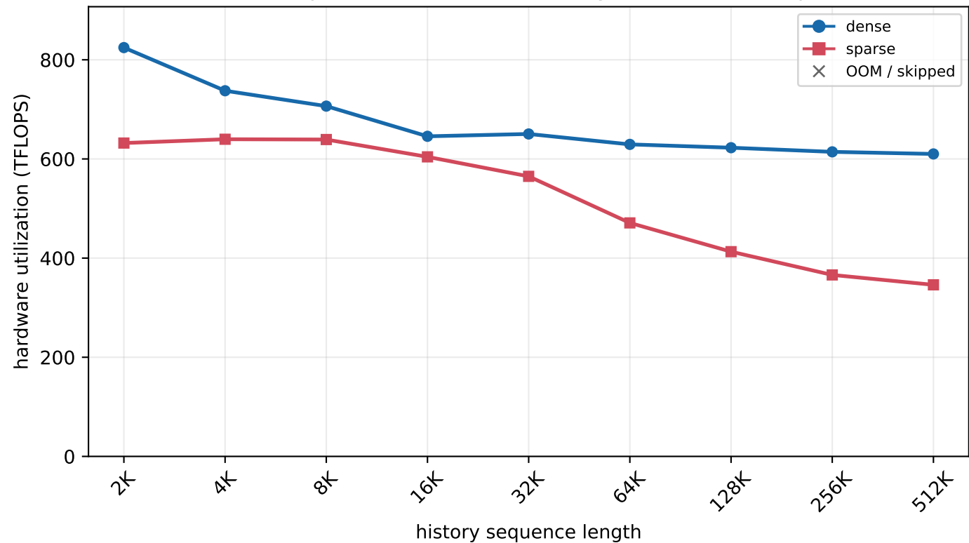
H800 MLA prefill - batch=8, new length=1K (chunked prefill)
