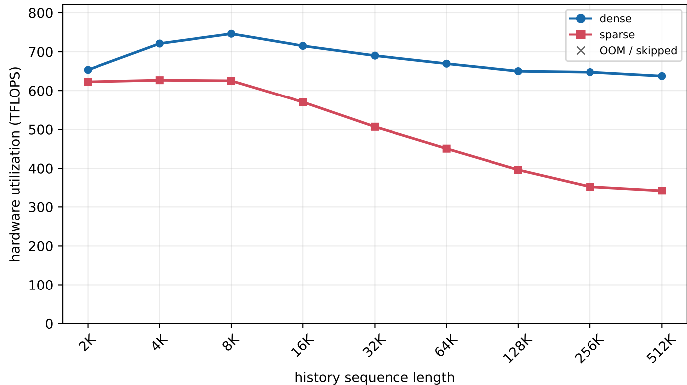
H800 MLA prefill - batch=8, new length=128 (chunked prefill)
