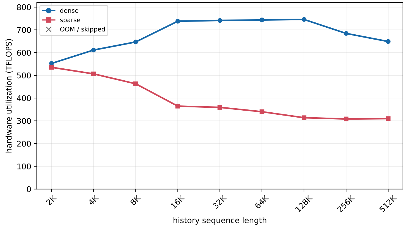
H800 MLA prefill - batch=8, new length=16 (chunked prefill)
