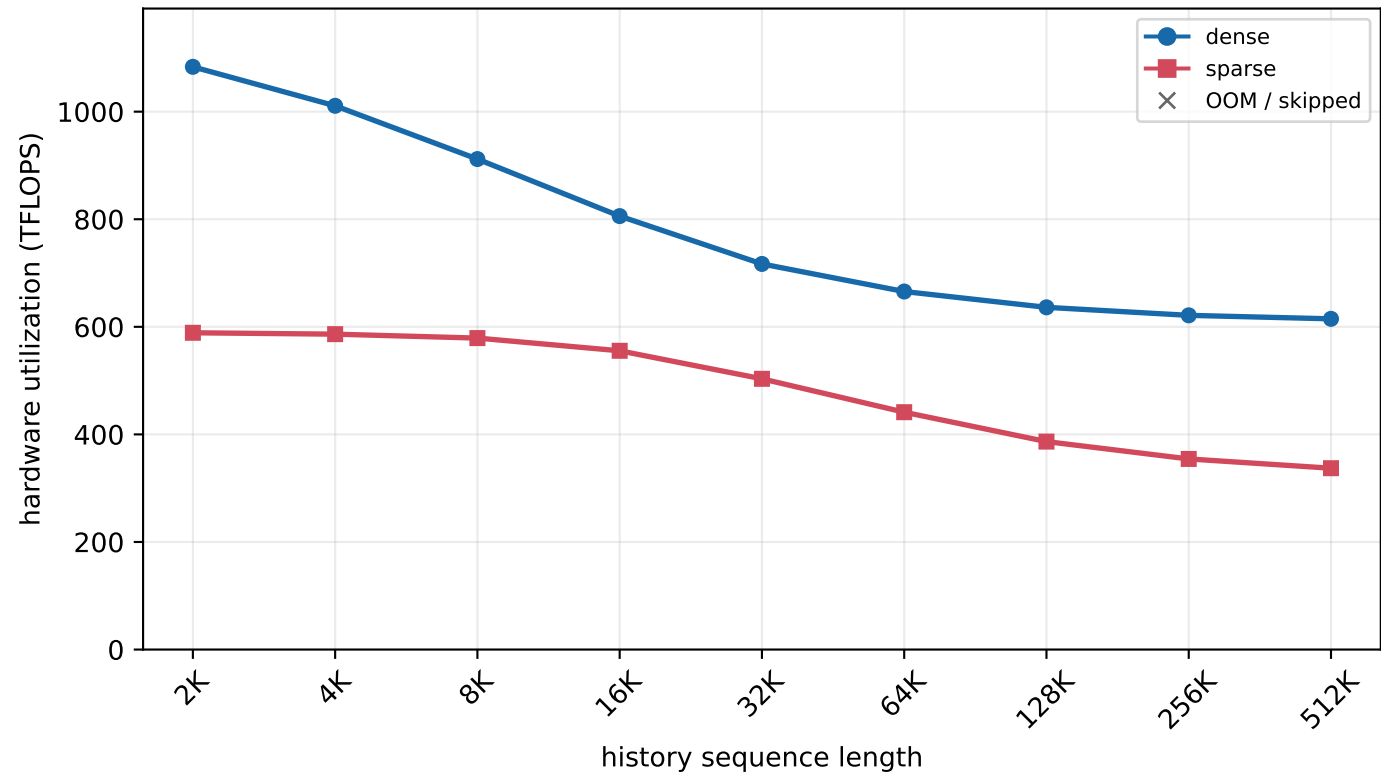
H800 MLA prefill - batch=8, new length=16K (chunked prefill)
