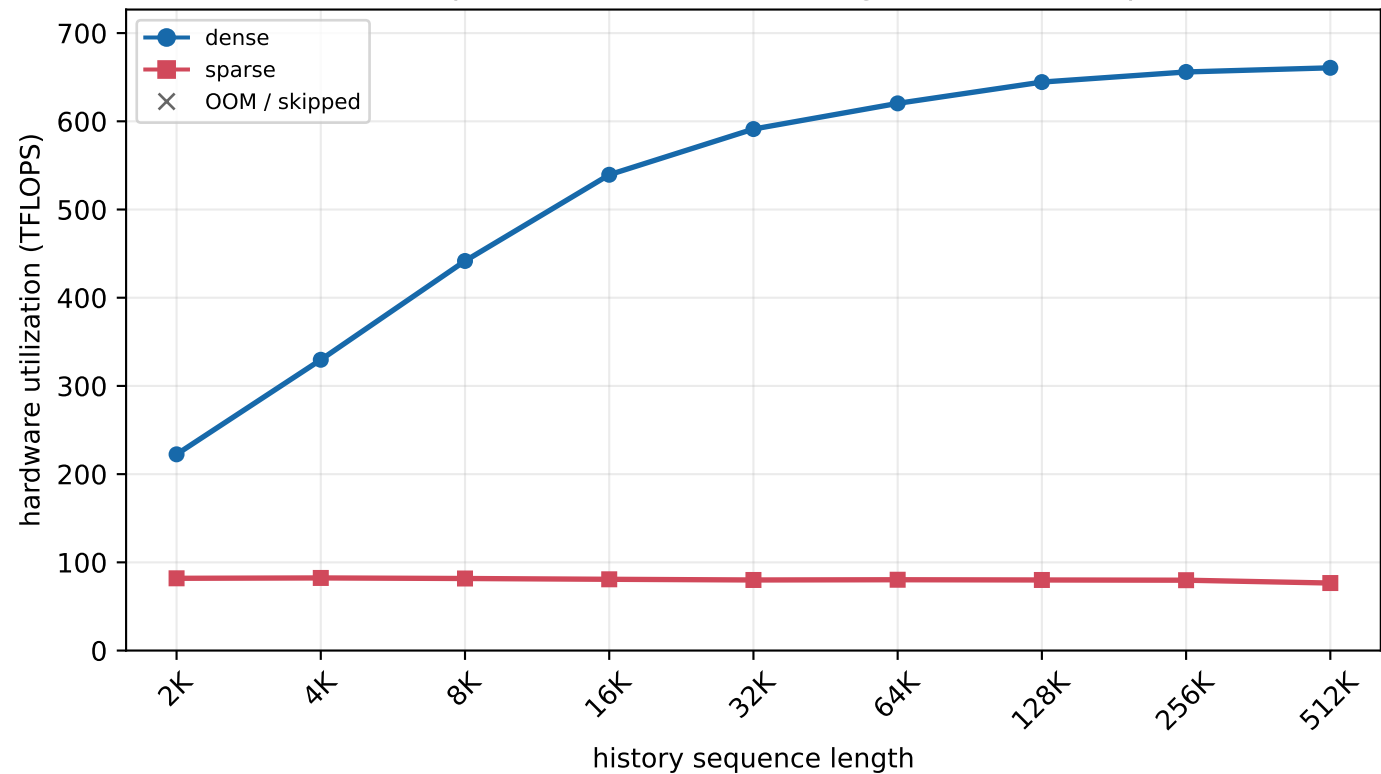
H800 MLA prefill - batch=8, new length=2 (chunked prefill)
