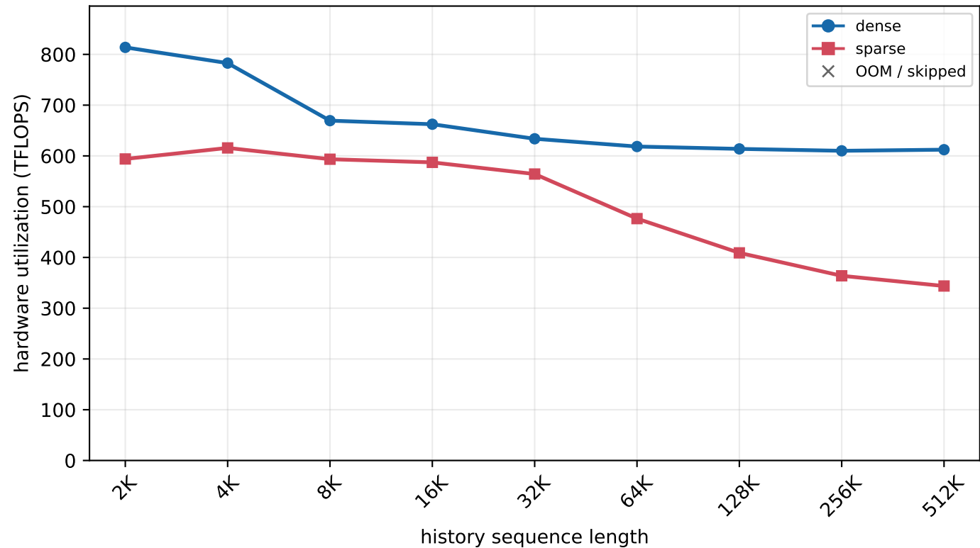
H800 MLA prefill - batch=8, new length=2K (chunked prefill)
