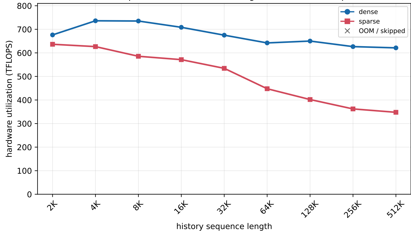
H800 MLA prefill - batch=8, new length=256 (chunked prefill)
