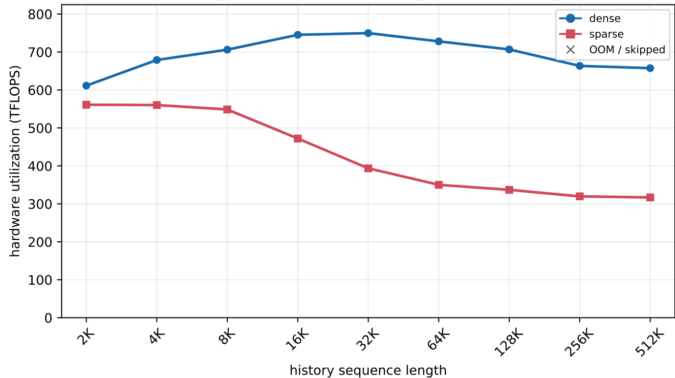
H800 MLA prefill - batch=8, new length=32 (chunked prefill)
