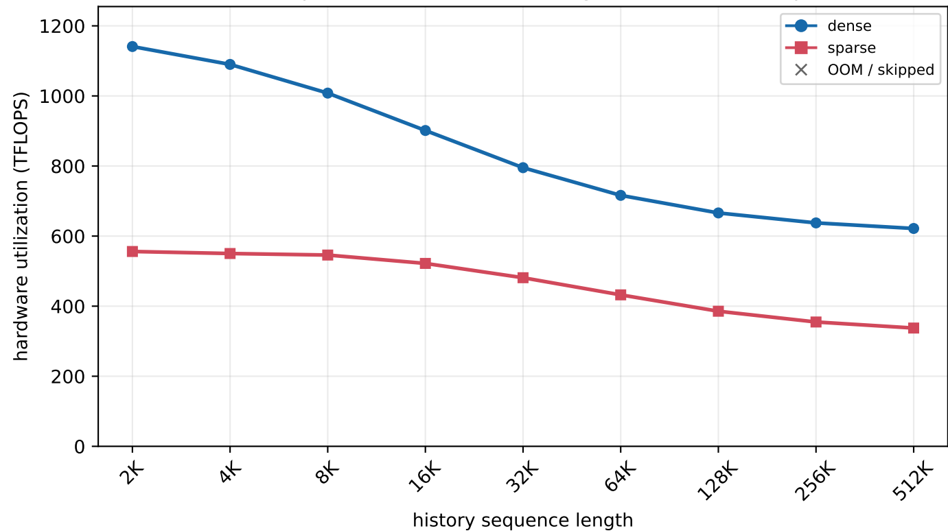
H800 MLA prefill - batch=8, new length=32K (chunked prefill)
