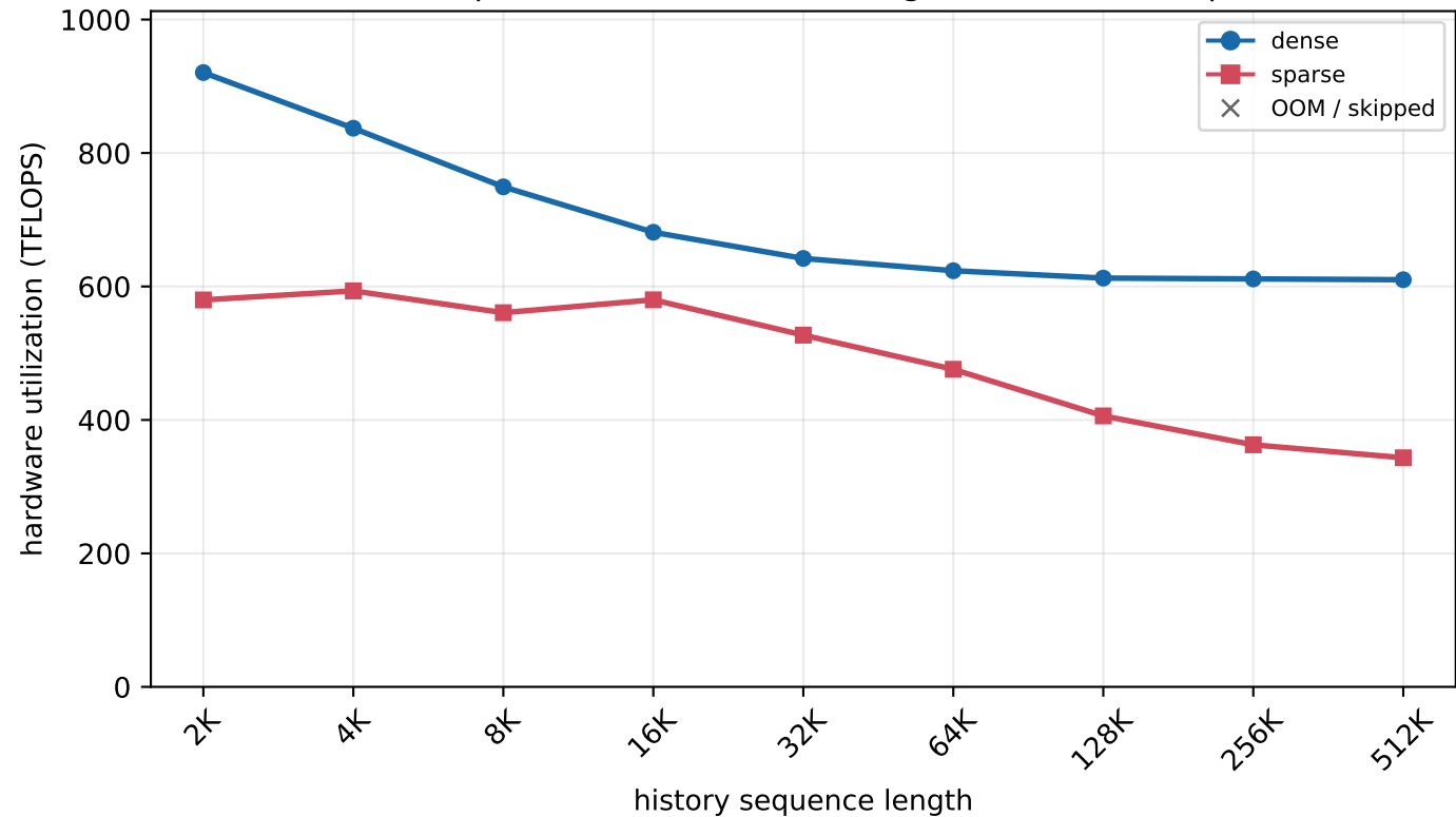
H800 MLA prefill - batch=8, new length=4K (chunked prefill)
