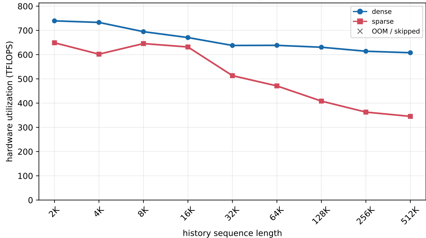
H800 MLA prefill - batch=8, new length=512 (chunked prefill)
