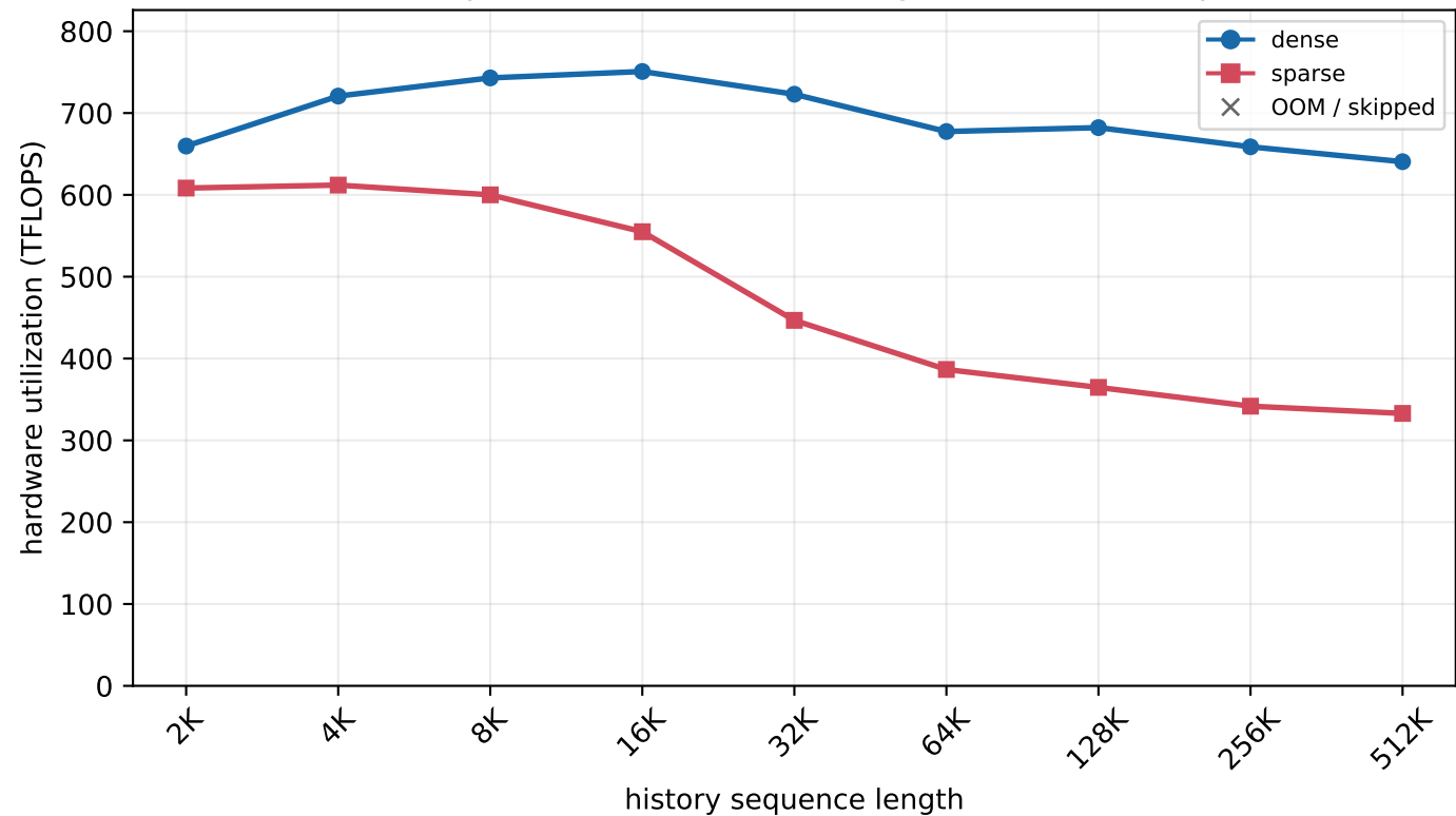
H800 MLA prefill - batch=8, new length=64 (chunked prefill)
