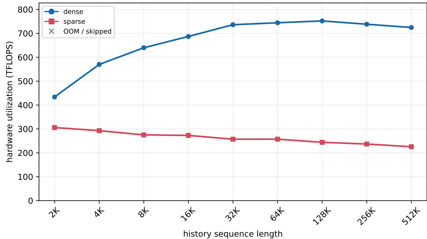
H800 MLA prefill - batch=8, new length=8 (chunked prefill)
