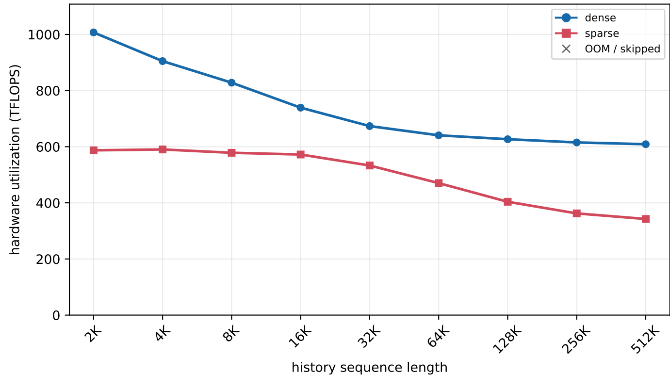
H800 MLA prefill - batch=8, new length=8K (chunked prefill)
