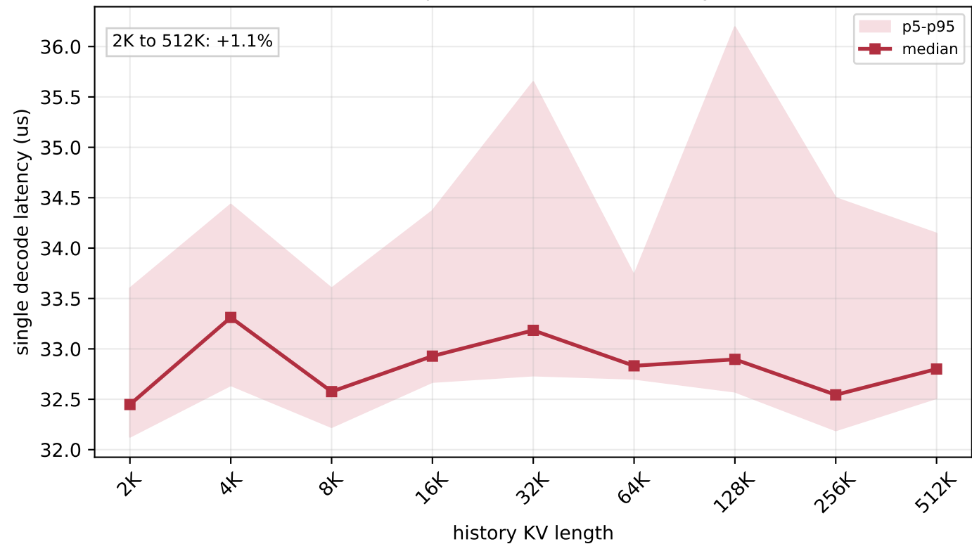
H800 FlashMLA sparse FP8 decode latency - batch=1
