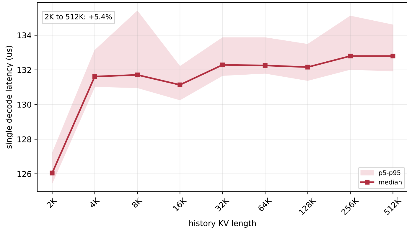
H800 FlashMLA sparse FP8 decode latency - batch=128
