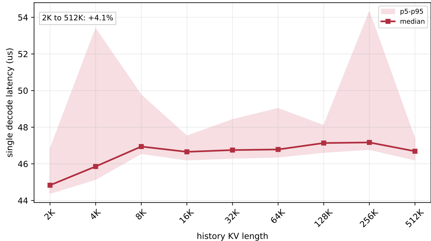
H800 FlashMLA sparse FP8 decode latency - batch=16
