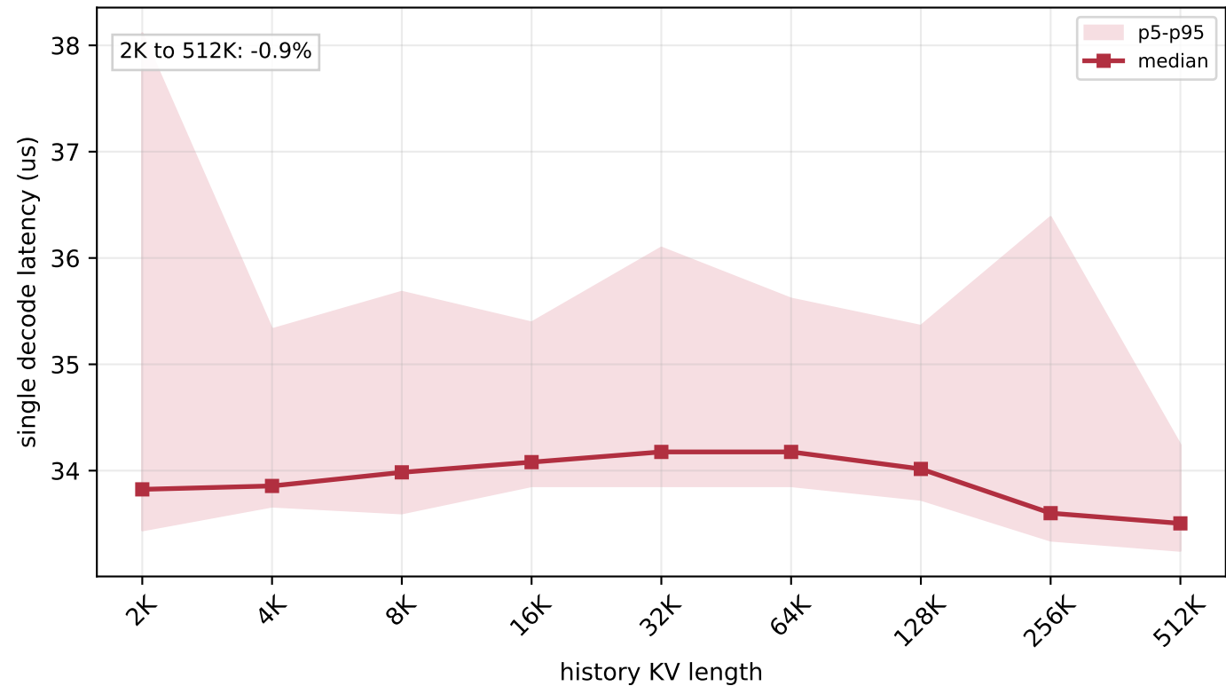
H800 FlashMLA sparse FP8 decode latency - batch=2
